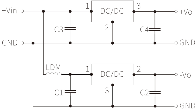
Fig 2: Parallel Application Circuit for Positive and Negative Outputs
