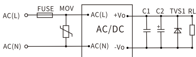
Figure 1 shows a normal application circuit
