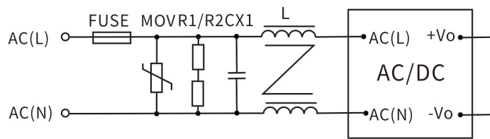
Figure 2 shows an EMC application circuit
