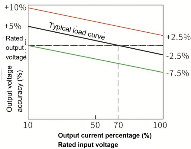
Error Envelope Curve
